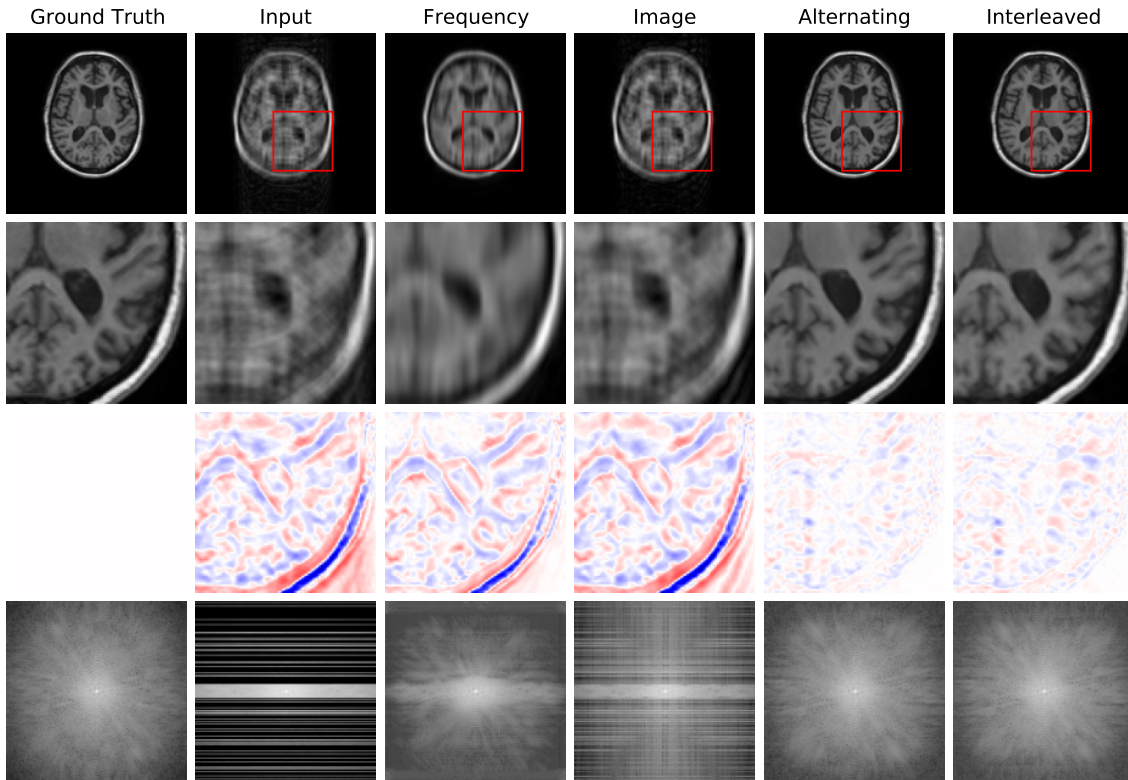
Figure 6: Example reconstructions from 4x undersampled, motion-corrupted data data, zoomed-in image patches, difference patches between reconstructions and ground truth images, and frequency space reconstructions. As in the motion corruption and undersampling examples, the Interleaved and Alternating architectures provide more accurate reconstructions of the ground truth images and reconstructing a more coherent k-space.
